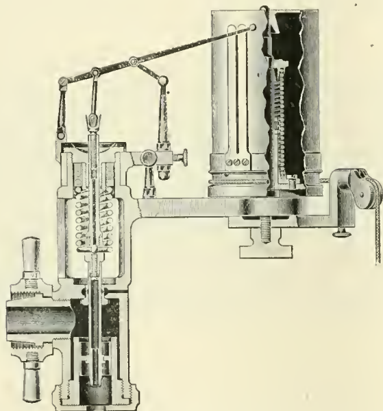
STAR IMPROVED INDICATOR.
